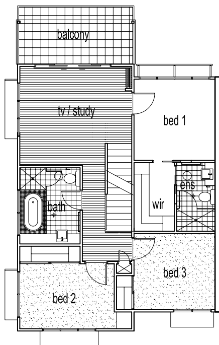
Level 1 floor plan
