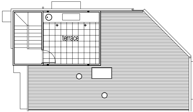
Roof plan
